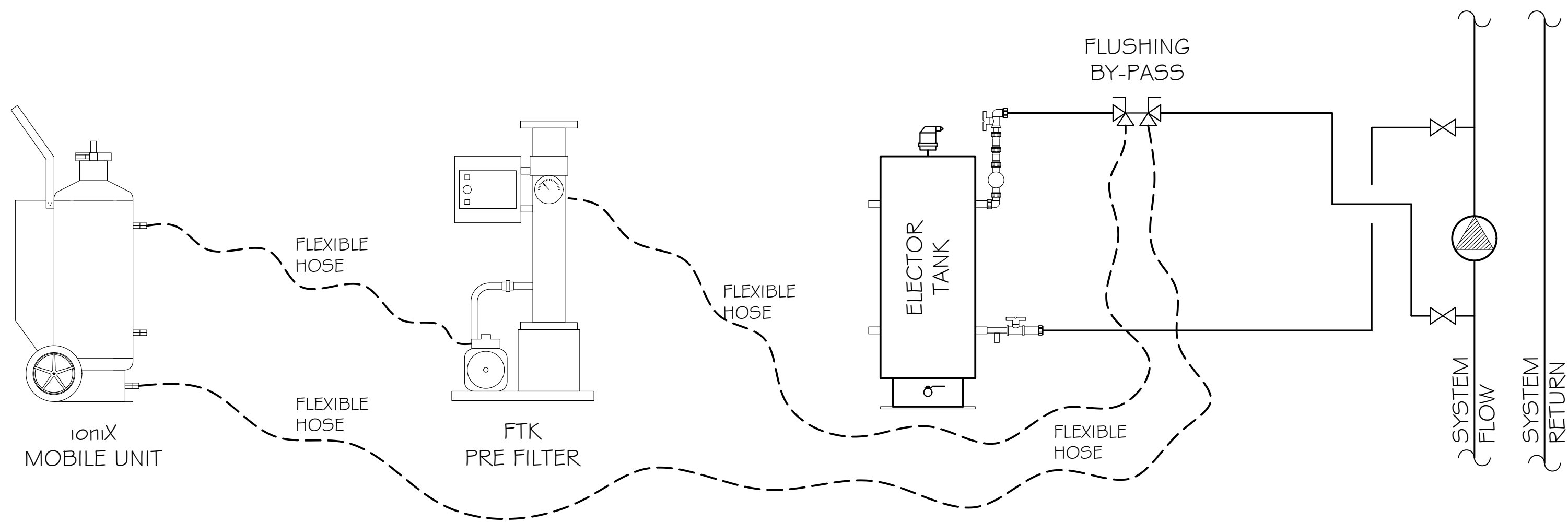
IN-LINE TREATMENT USING ioniX MOBILE + FTK PRE FILTER UTILISING FLUSHING BY-PASS FROM ELECTOR TANK INSTALLATION
